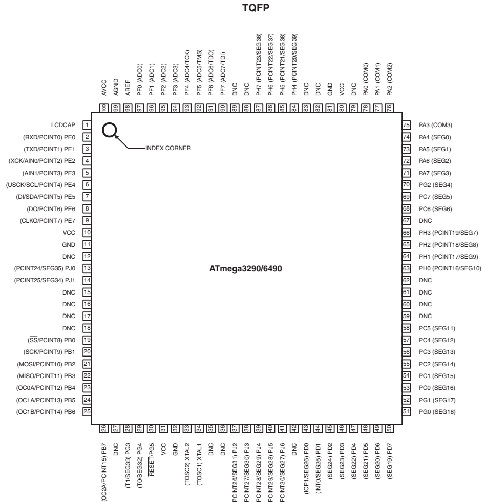
Figure 1. Pinout ATmega3290/6490
