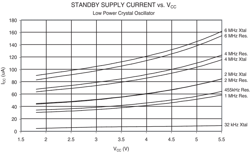
Standby Supply Current Figure 155. Standby Supply Current vs. V_{CC} (Low Power Crystal Oscillator)
