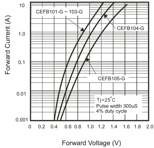
Fig.2 - Forward Characteristics
