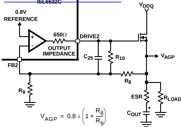
FIGURE 7. COMPENSATION AND OUTPUT VOLTAGE SELECTION OF THE LINEAR
