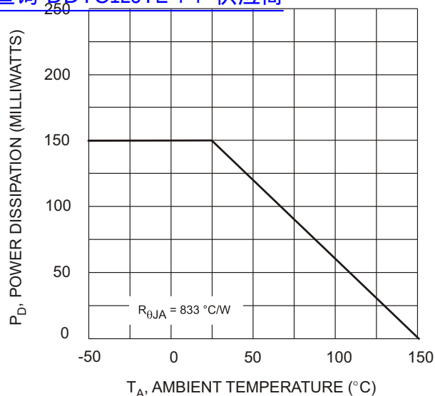
Fig. 1 Derating Curve
