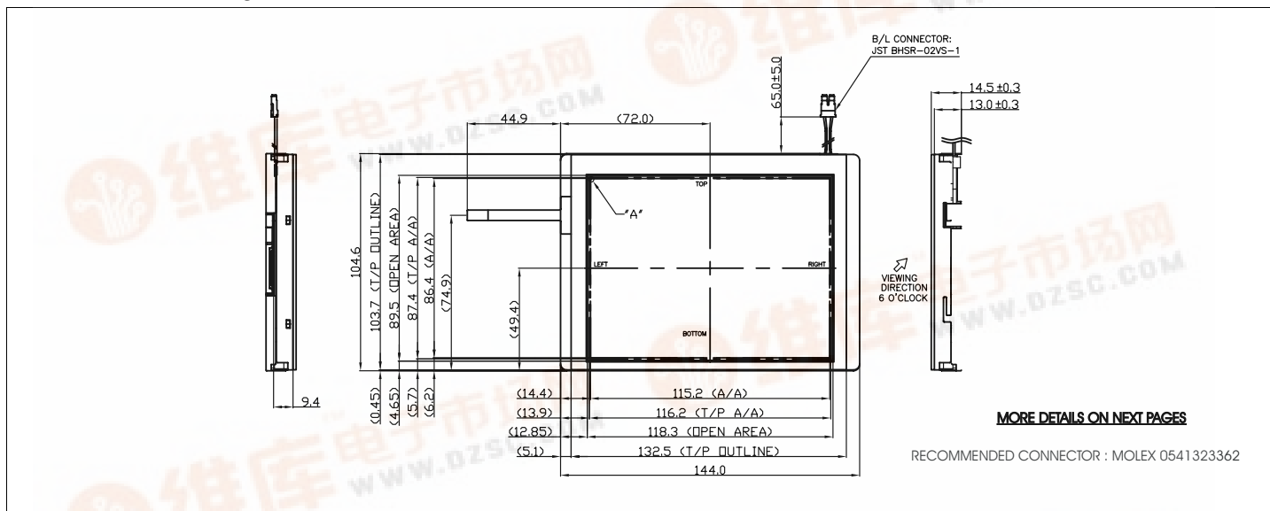
Dimensional Drawing
