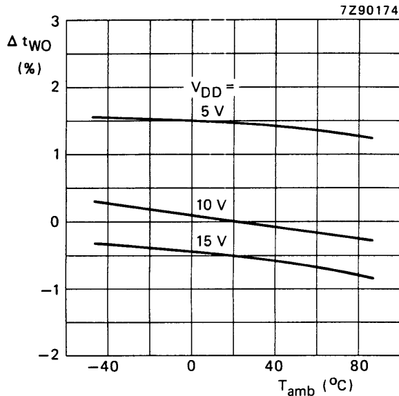
(a) R_t = 100 \text{ k}\Omega ; C_t = 100 \text{ nF} .
