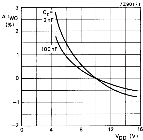
Fig.8 Typical normalized change in output pulse width as a function of the supply voltage at T_{amb} = 25^\circ\text{C} ; 0% at V_{DD} = 10 \text{ V} ; R_t = 100 \text{ k}\Omega .
