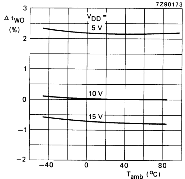
(b) R_t = 100 \text{ k}\Omega ; C_t = 2 \text{ nF} .
