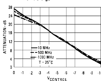
Attenuation of LG1 and G1 in Cascade vs. Control Voltage
