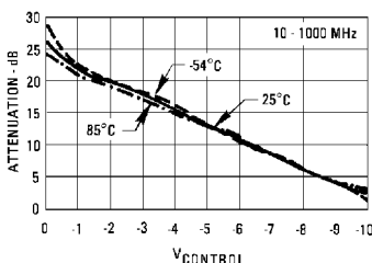
Attenuation of LG1 and G2 in Cascade vs. Control Voltage
