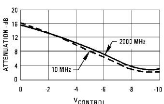
Attenuation of LG1 and G2 in Cascade vs. Control Voltage
