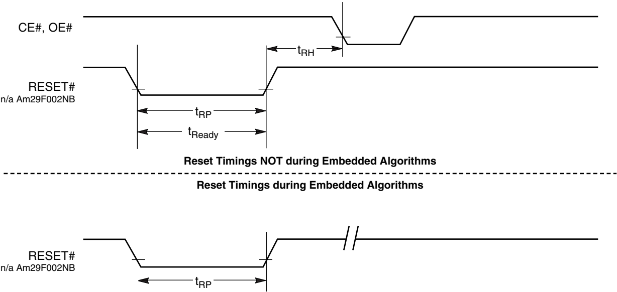
Figure 10. RESET# Timings
