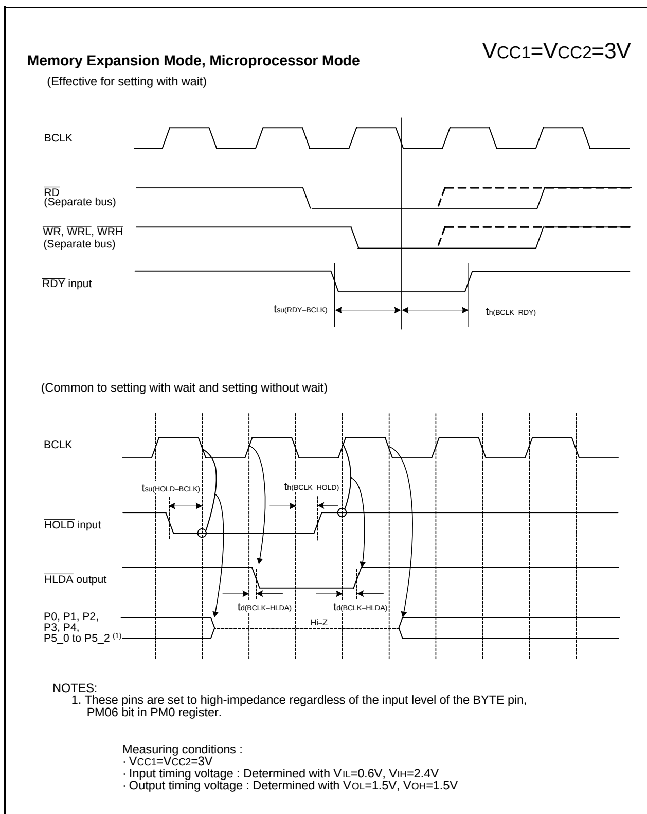
Figure 5.11 Timing Diagram (3)
