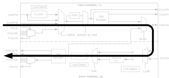
Figure 6: Local (Analog) Loopback
