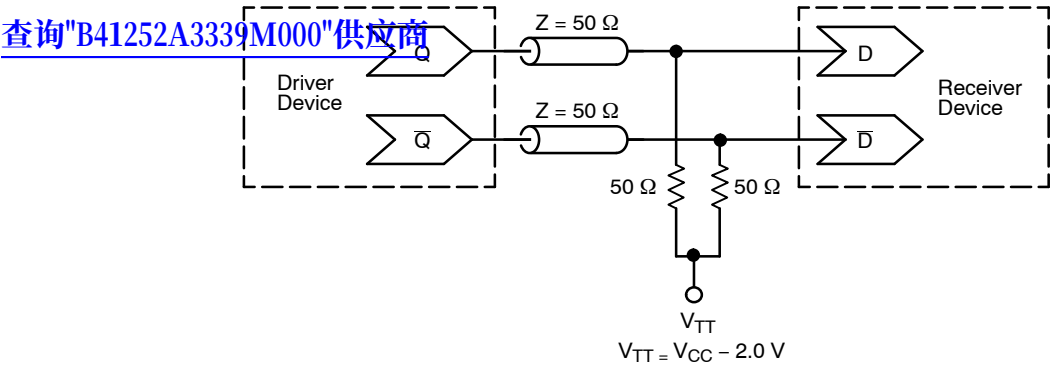
Figure 21. Typical Termination for Output Driver and Device Evaluation (See Application Note AND8020/D – Termination of ECL Logic Devices.)
