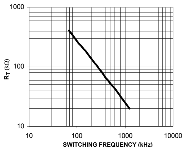
FIGURE 21. R_T vs SWITCHING FREQUENCY
