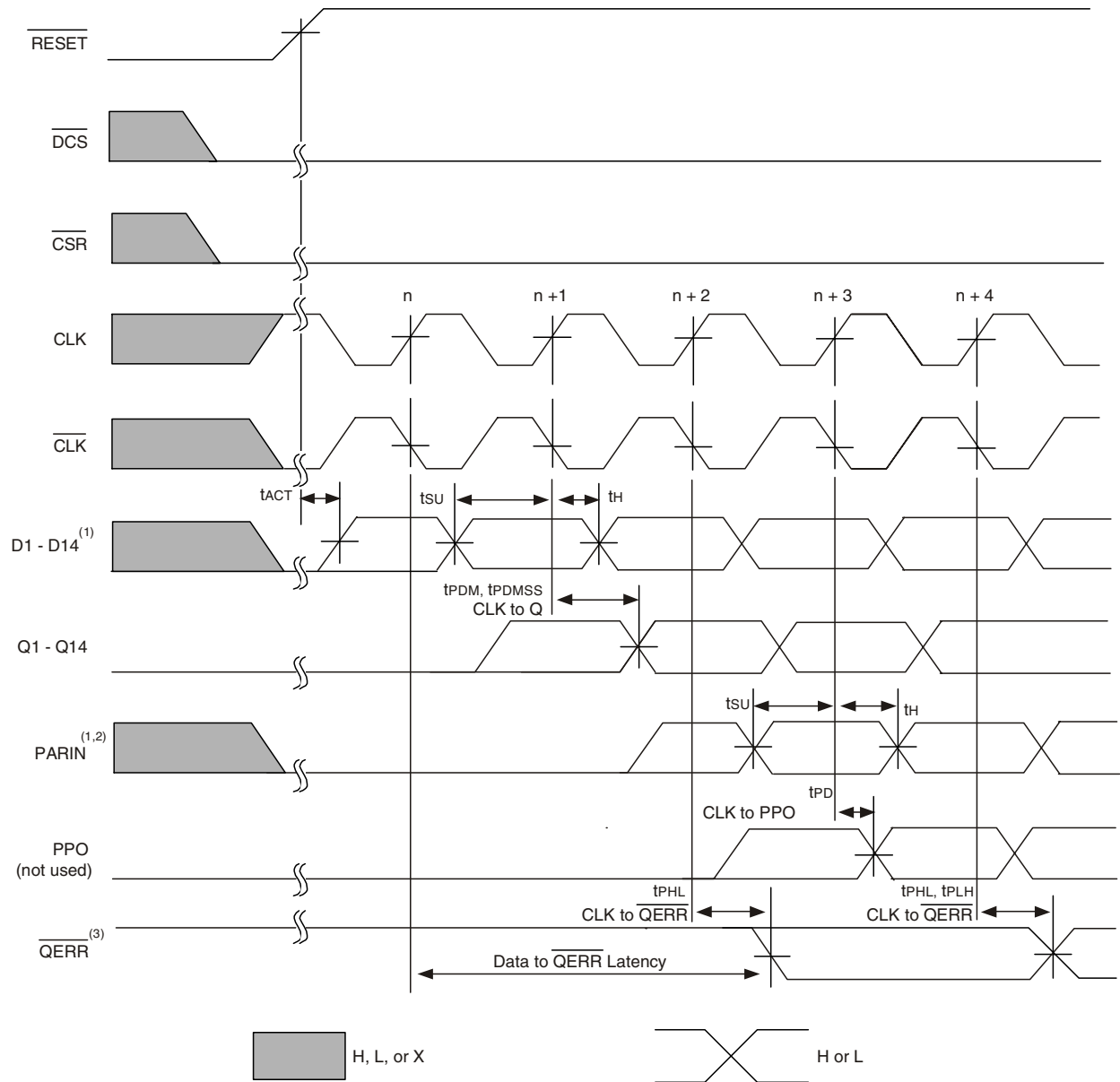
Timing Diagram for the Second IDT74SSTUAE32866A (1:2 Register-B Configuration) Device Used in a Pair; C0 = 1, C1 = 1, \overline{\text{RESET}} Switches from L to H
