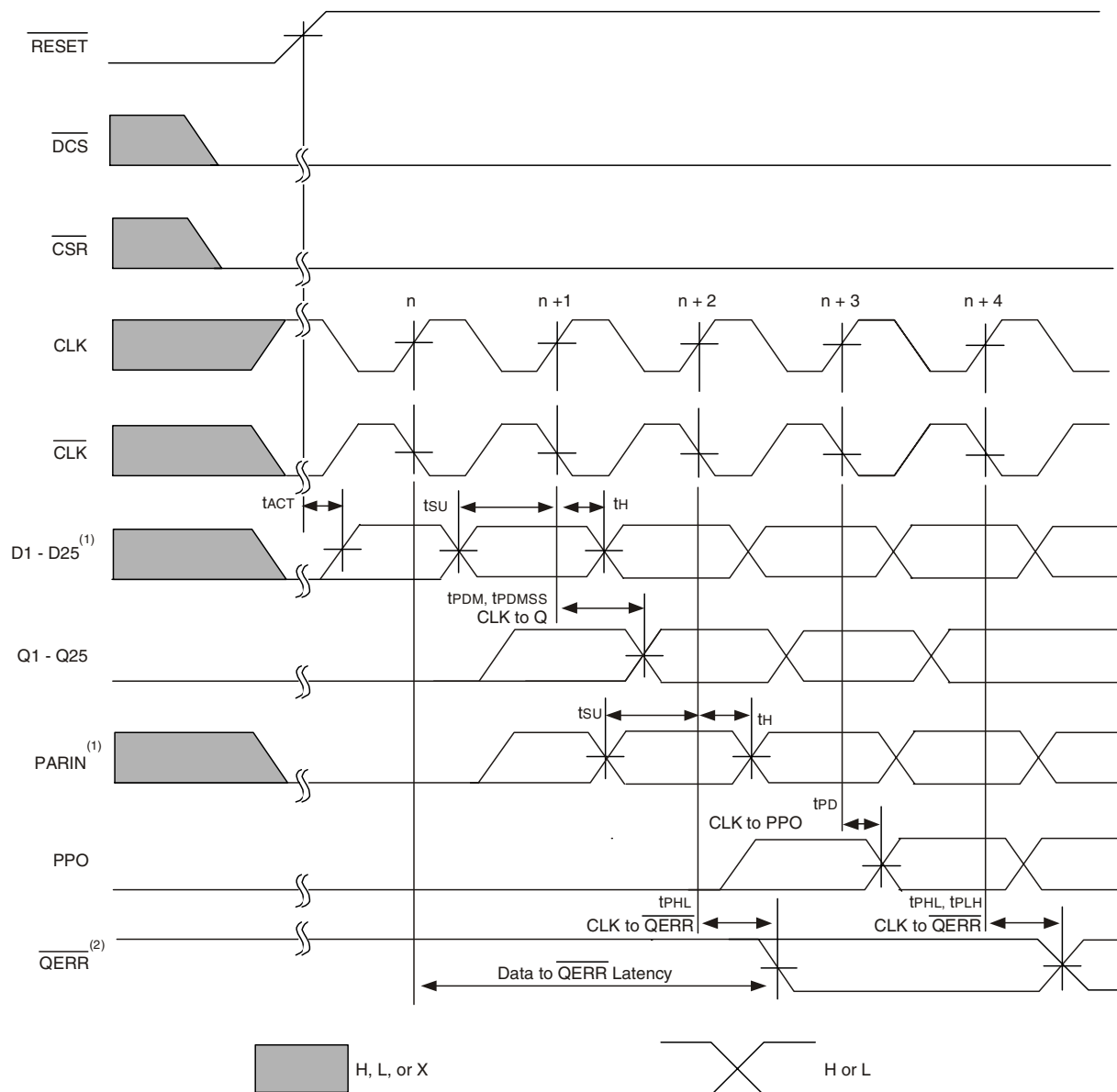
Timing Diagram for IDT74SSTUAE32866A Used as a Single Device; C0 = 0, C1 = 0, RESET Switches from L to H
