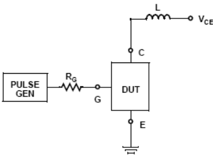
Figure 17. Inductive Switching Test Circuit
