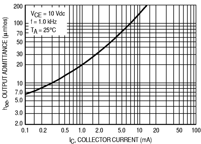
Figure 16. Output Admittance
