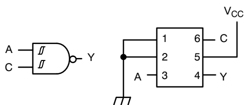
Figure 3. 2-Input NAND (When B = "L")
