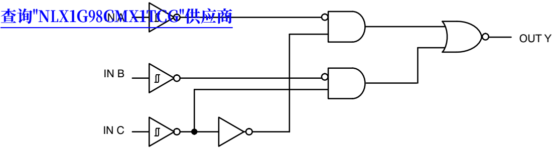
Figure 1. Function Diagram
