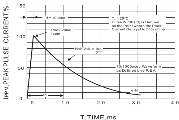
Fig.3 PULSE WAVEFORM
