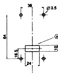
PANEL CUTOUT & DRILLING DETAILS FOR MOUNTING TO PANEL SURFACE
