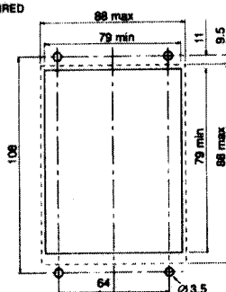
PANEL CUTOUT & DRILLING DETAILS FOR UNDER PANEL MOUNTING
