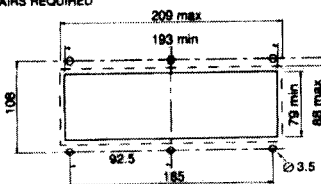
PANEL CUTOUT & DRILLING DETAILS FOR UNDER PANEL MOUNTING
