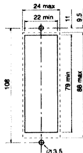
PANEL CUTOUT & DRILLING DETAILS FOR UNDER PANEL MOUNTING
