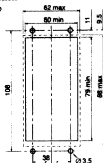
PANEL CUTOUT & DRILLING DETAILS FOR UNDER PANEL MOUNTING
