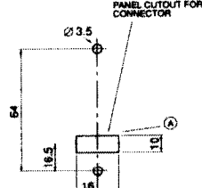
PANEL CUTOUT & DRILLING DETAILS FOR MOUNTING TO PANEL SURFACE
