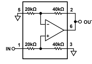
Figure 54. Noninverting Amplifier, Gain = 2
