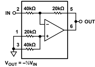
Figure 52. Inverting Amplifier, Gain = -1/2
