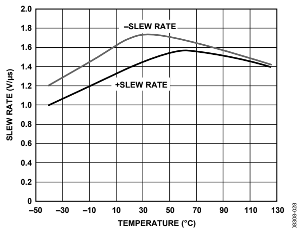
Figure 28. Slew Rate vs. Temperature, V_{IN} = 20\text{ V p-p} , 1\text{ kHz}
