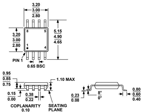
Figure 58. 8-Lead Mini Small Outline Package [MSOP]
