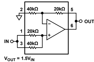
Figure 53. Noninverting Amplifier, Gain = 1.5
