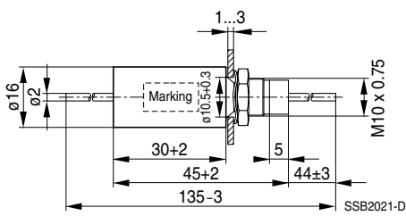
Figure 1, B85121A****C160
