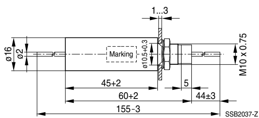
Figure 2, B85121A****B160
