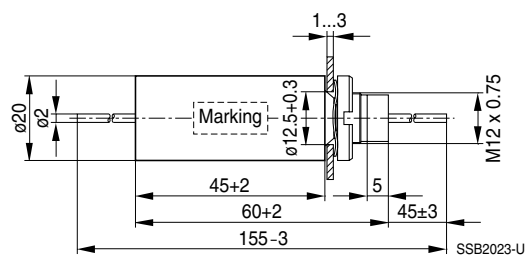
Figure 2, B85121A****B250
