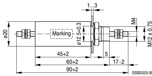
Figure 1, B85121A****A250
