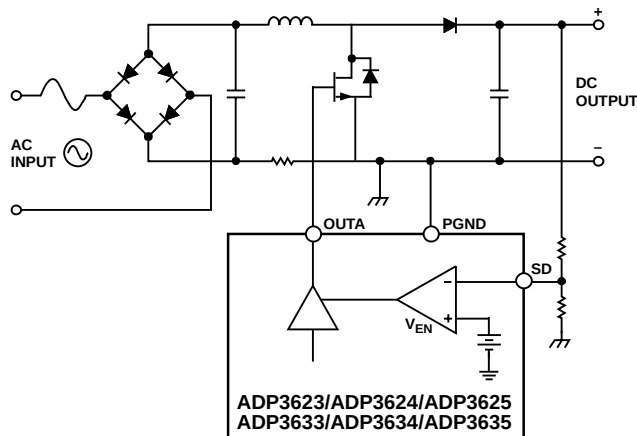
Figure 22. Shutdown Function Used for Redundant OVP
