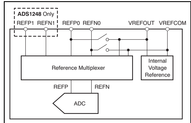
Figure 32. Reference Input Multiplexer
