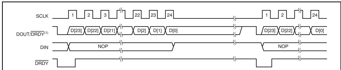
Figure 50. Data Retrieval with the DRDY MODE Bit = 1 (Enabled)
