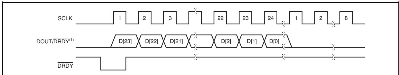
Figure 49. Data Retrieval with the DRDY MODE Bit = 0 (Disabled)
