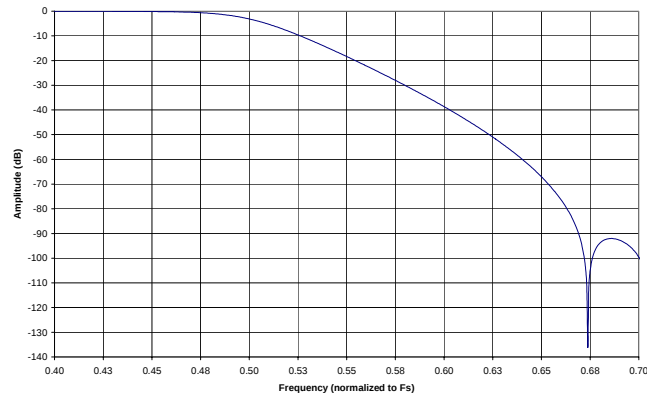
Figure 32. Double-Speed Mode Transition Band
