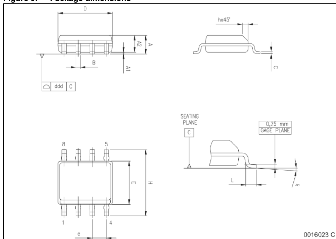
Figure 9. Package dimensions
