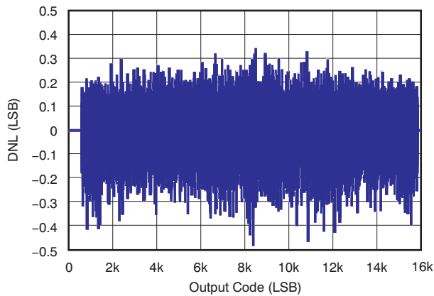
DIFFERENTIAL NONLINEARITY
