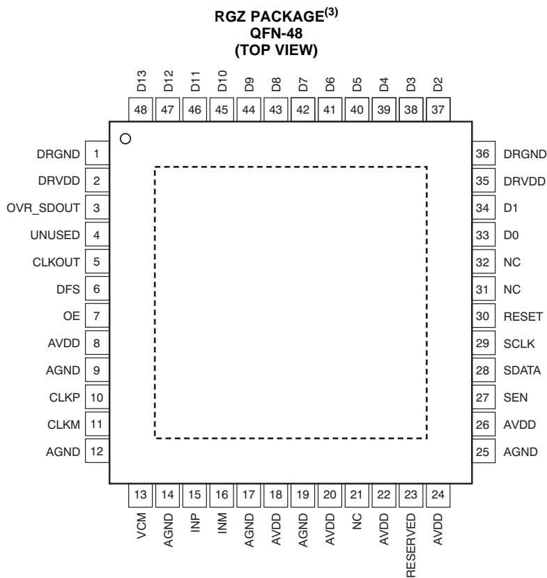
Figure 13. ADS414x CMOS Pinout (2)
