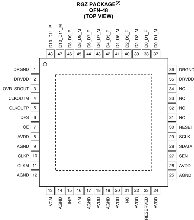
Figure 12. ADS412x LVDS Pinout (2)
