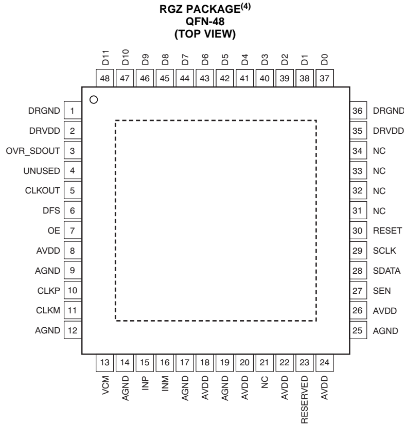
Figure 14. ADS412x CMOS Pinout (2)
