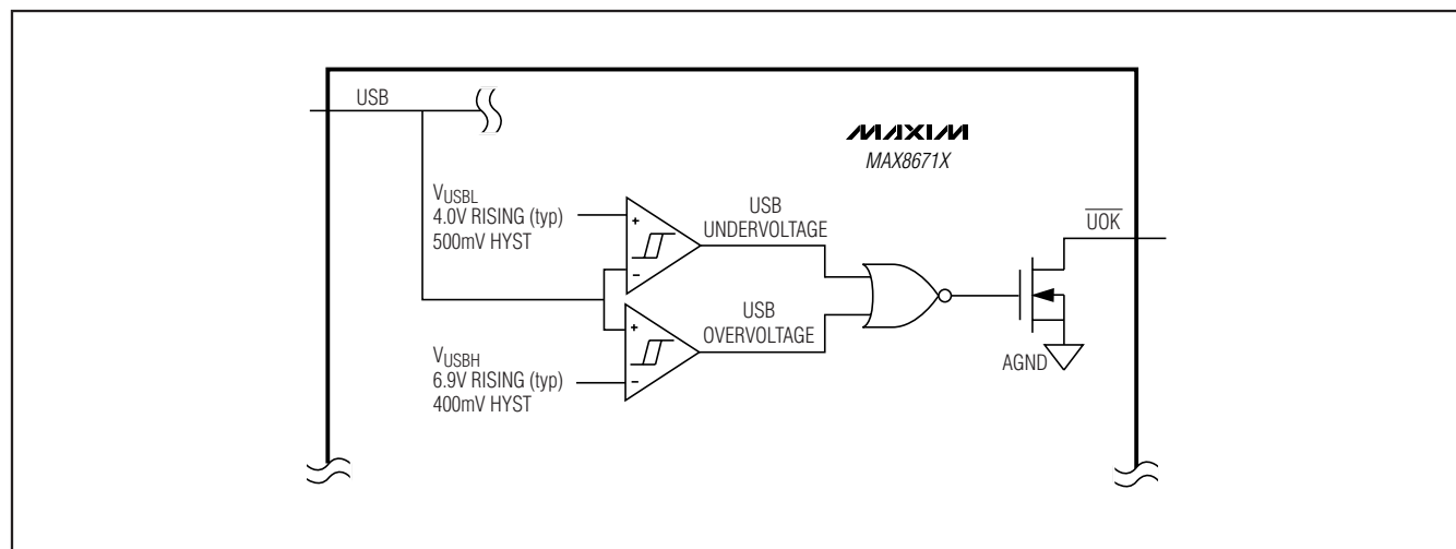
Figure 3. USB Power-OK Logic
