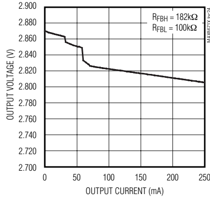
REG1 LOAD REGULATION
