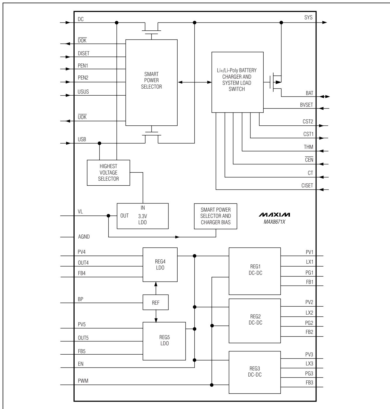
Figure 2. Functional Diagram
