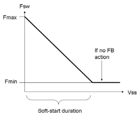
Figure 42. Soft-Start Behavior
