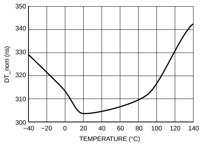
Figure 12. T_dead_A
