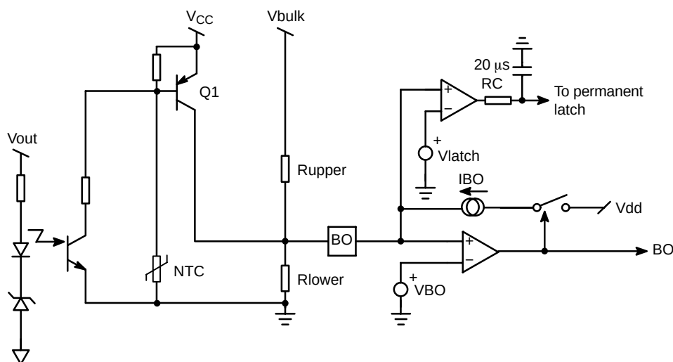
Figure 47. Adding a comparator on the BO pin offers a way to latch-off the controller.
