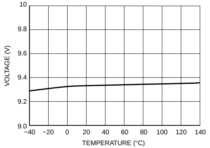
Figure 4. VCCmin
