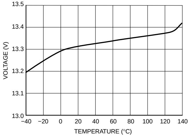
Figure 3. VCCon A
