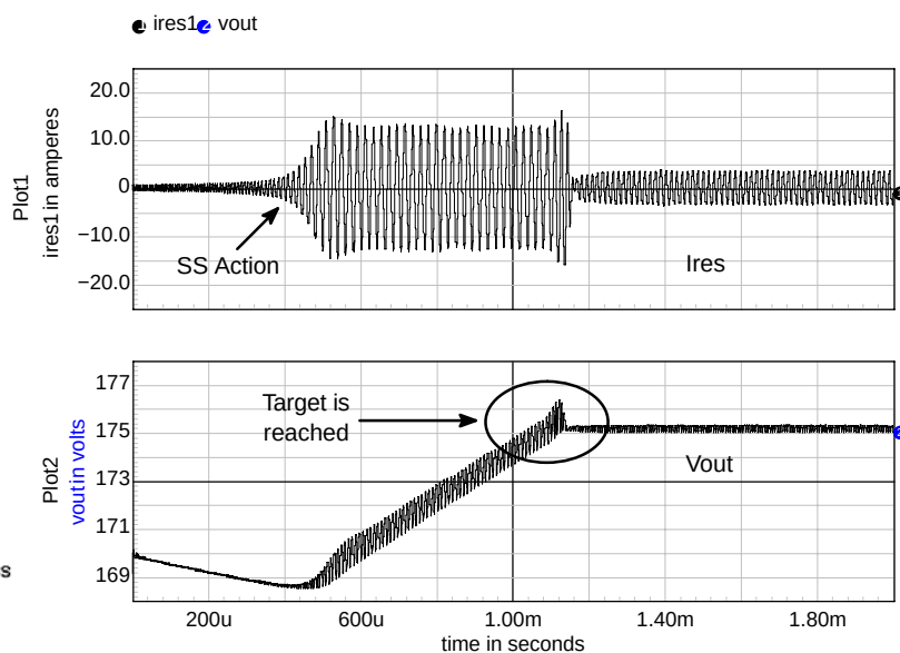
Figure 43. A Typical Startup Sequence on an LLC Converter
