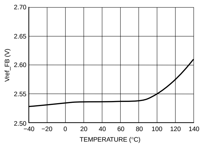
Figure 22. Reference (Vref_FB)
