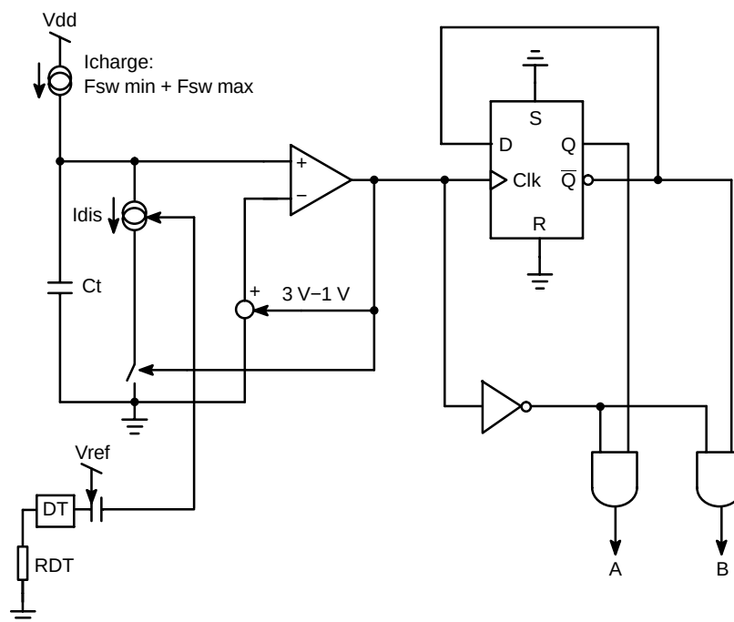
During the discharge time, the clock comparator is high and unvalidates the AND gates: both outputs are low. When the comparator goes back to the high level, during the timing capacitor C_t recharge time, A and B outputs are validated. By connecting a resistor RDT to ground, it creates a current whose image serves to discharge the C_t capacitor: we control the deadtime. The typical range evolves between 150 ns (RDT = 30 k \Omega ) and 1.0 \mu s (RDT = 600 k \Omega ). Figure 44 shows the typical waveforms obtained on the output.
