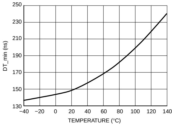
Figure 11. T_dead_min A
