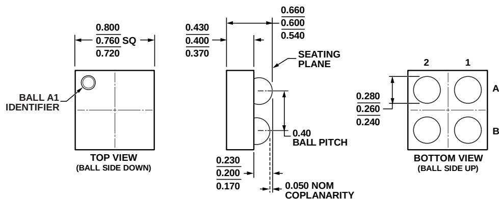
Figure 50.4-Ball Wafer Level Chip Scale Package [WLCSP] (CB-4-3)
