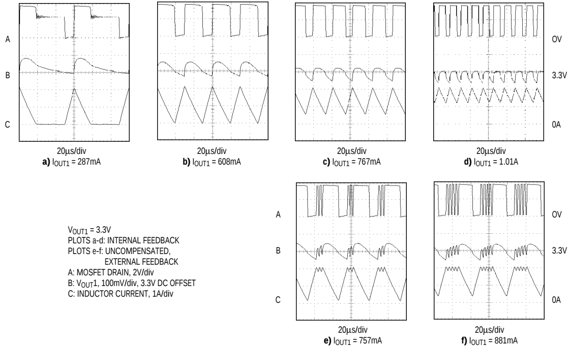
Figures 3a–3f. MAX863 Switching Waveforms During Transition into Continuous Conduction
