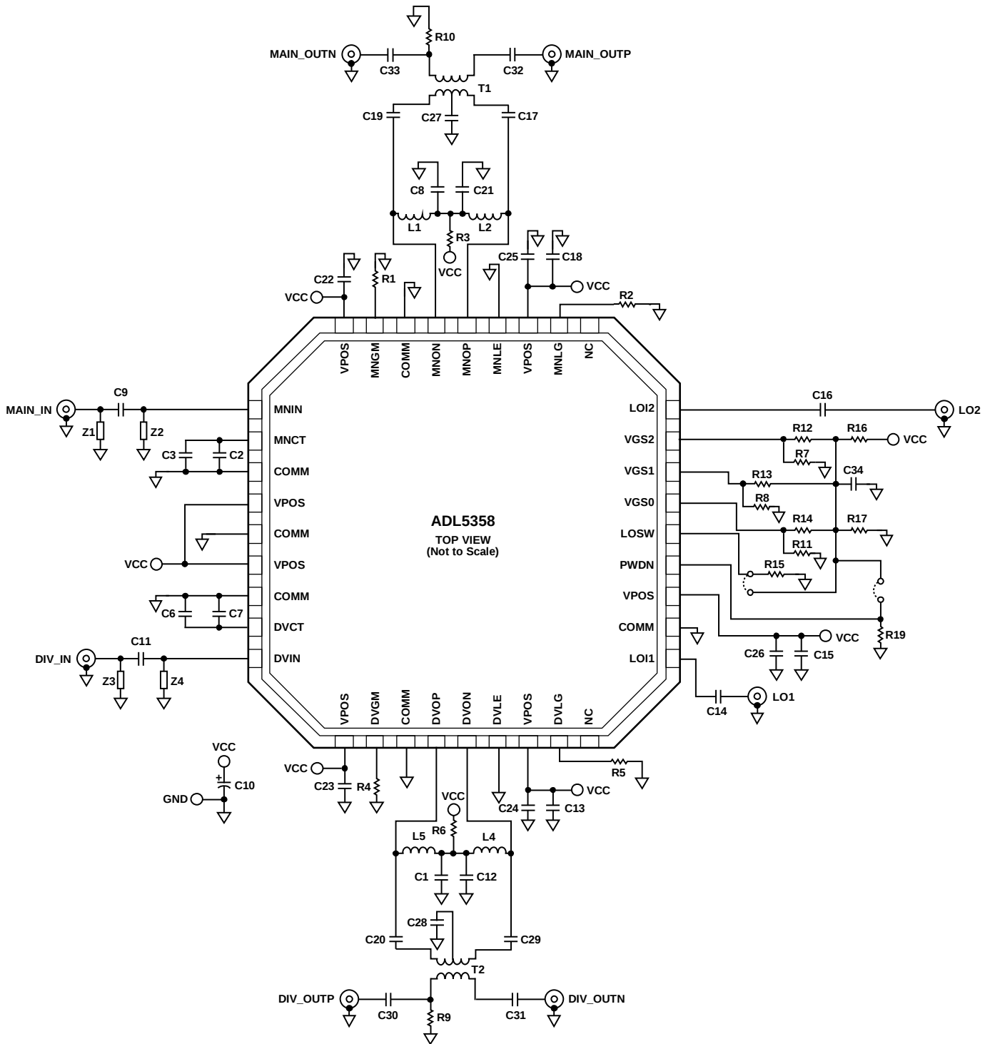
Figure 54. Evaluation Board Schematic
