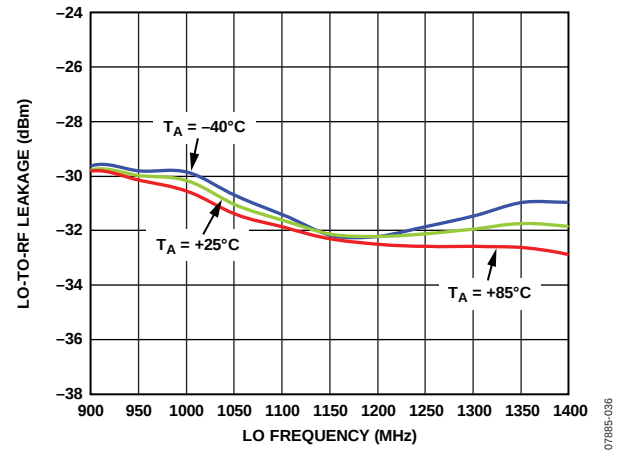
Figure 36. LO-to-RF Leakage vs. LO Frequency
