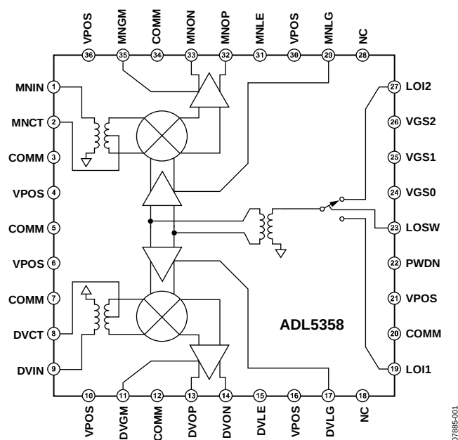
Figure 52. Simplified Schematic
