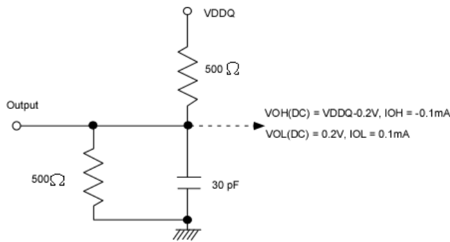
(Fig.1) DC Output Load circuit
