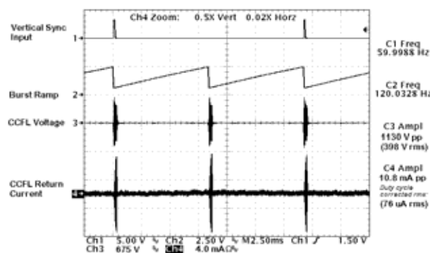
Figure 4 – 2% Burst Duty Cycle
