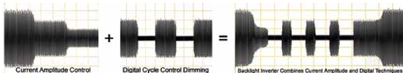
Figure 2 – LXM1614E Combines Current Amplitude and Digital Techniques
