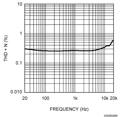
THD+N vs Frequency V_{DD} = 5V, R_L = 3\Omega, P_O = 600mW
