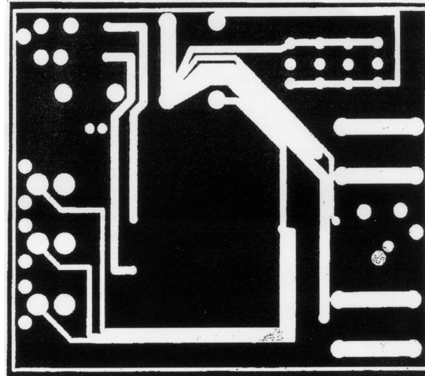
FIGURE 8. Inner Layer (3)
