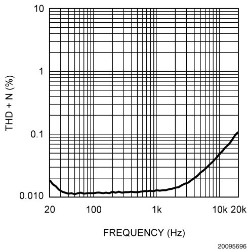
THD+N vs Frequency V_{DD} = 3V, R_L = 32\Omega, P_O = 20mW, SE
