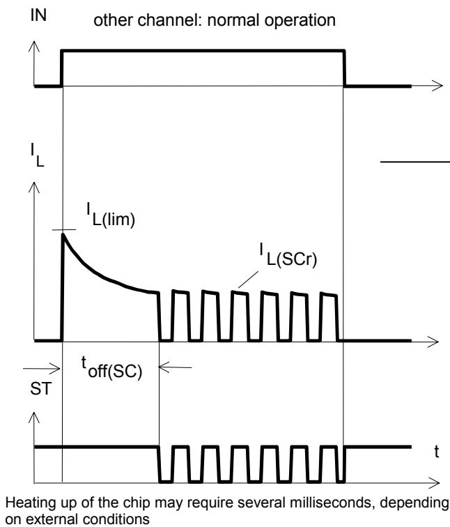
Figure 4a: Overtemperature:
