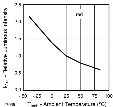
Figure 7. Relative Luminous Intensity vs. Amb. Temperature
