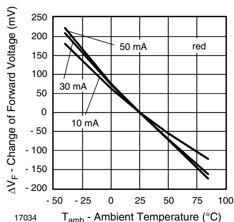
Figure 9. Change of Forward Voltage vs. Ambient Temperature
