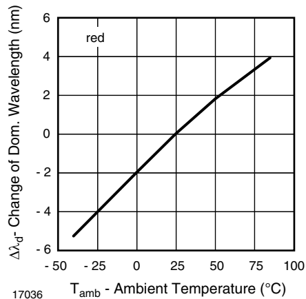
Figure 8. Change of Dominant Wavelength vs. Ambient Temperature
