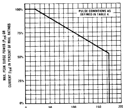
FIGURE 3 PULSE DERATING CURVE
