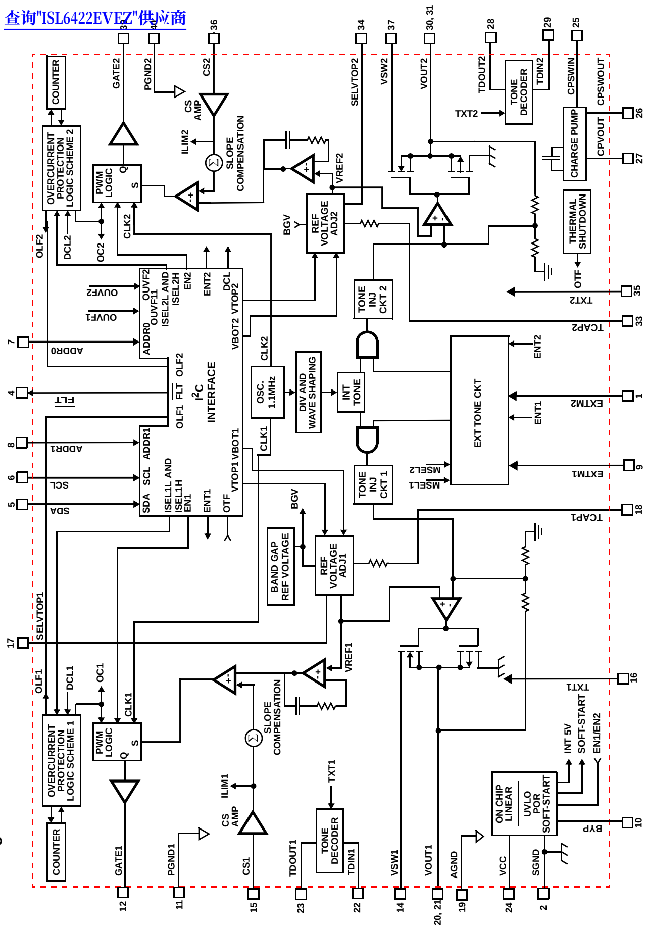
Block Diagram
