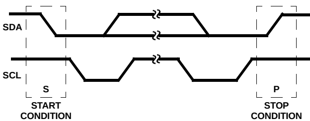
FIGURE 5. START AND STOP WAVEFORMS
