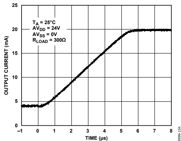
Figure 62. 4 mA to 20 mA Output Current Step
