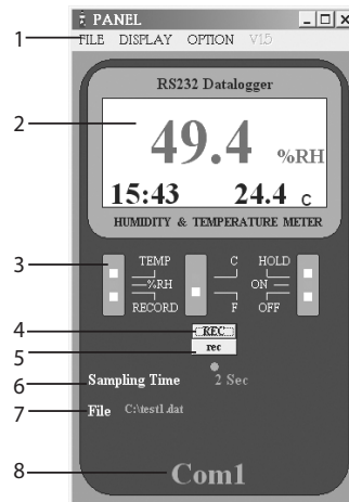
PANEL Software
