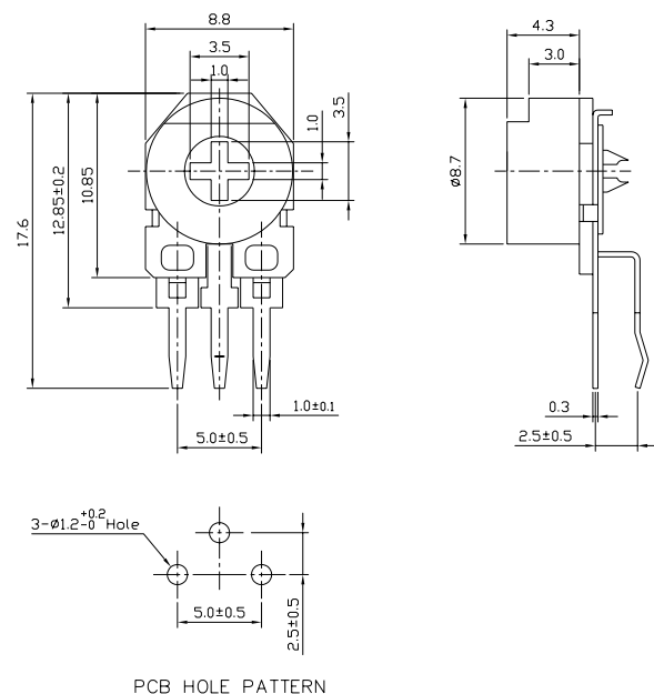
Model 37W (Side Adjust)
