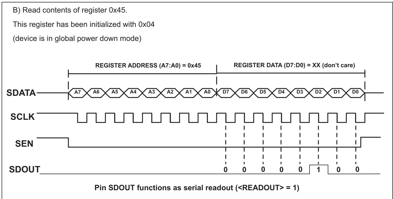
Figure 7. Serial Readout
