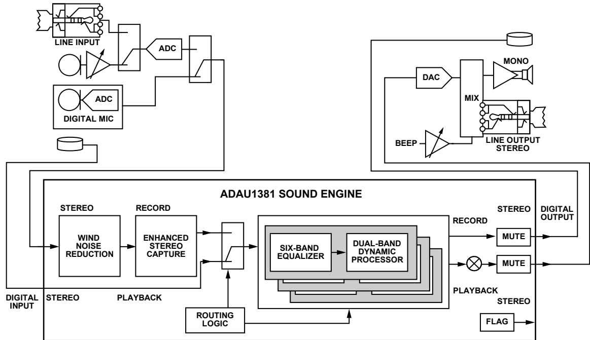
Figure 52. Sound Engine Signal Processing Flow
