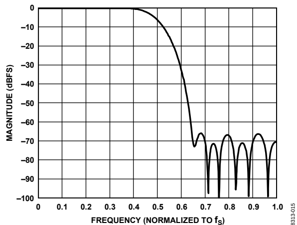
Figure 15. DAC Interpolation Filter, 64x Oversampling, Normalized to f_s
