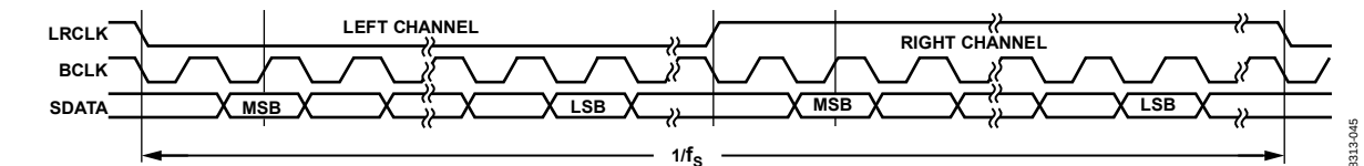
Figure 47. I²S Mode—16 Bits to 24 Bits per Channel
