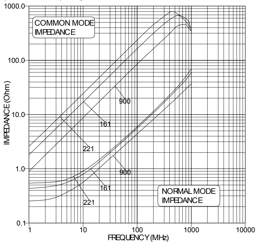
P7500-3216 impedance vs frequency characteristics
