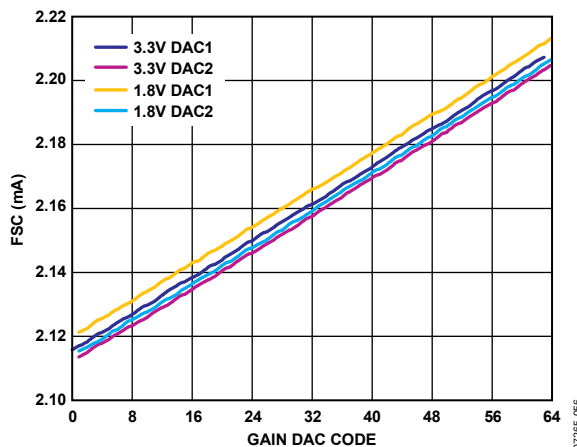
Figure 86. Typical DAC Gain Characteristics
