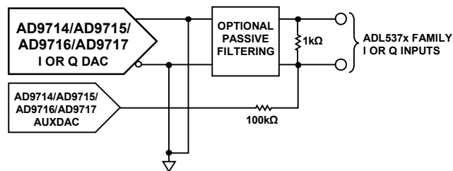
Figure 95. Typical Use of Auxiliary DACs When DC Coupling to Quadrature Modulator ADL537x Family
