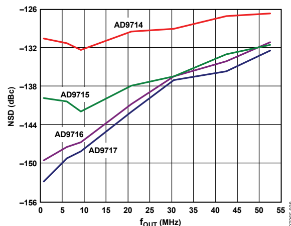
Figure 40. AD9714/AD9715/AD9716/AD9717 Noise Spectral Density at 1.8 V
