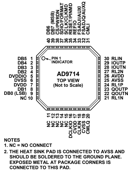
Figure 5. AD9714 Pin Configuration
