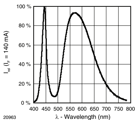
Figure 6. Relative Spectral Emission
