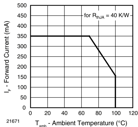
Figure 4. Max. Permissible Forward Current vs. Ambient Temperature
