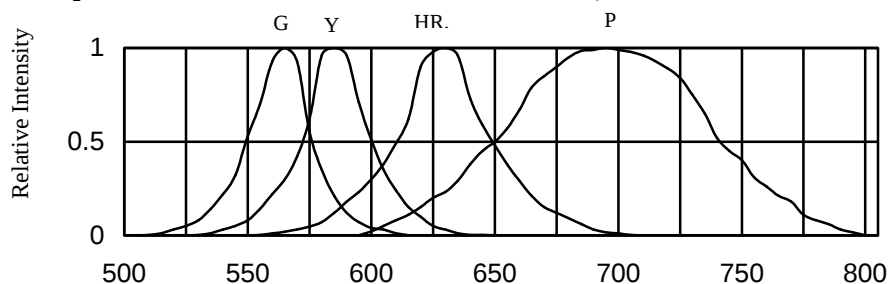
FIG.1 RELATIVE LUMINOUS INTENSITY VS. WAVELENGTH
