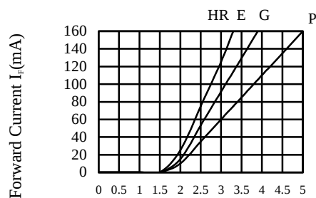
FIG.4 FORWARD CURRENT VS. FORWARD VOLTAGE
