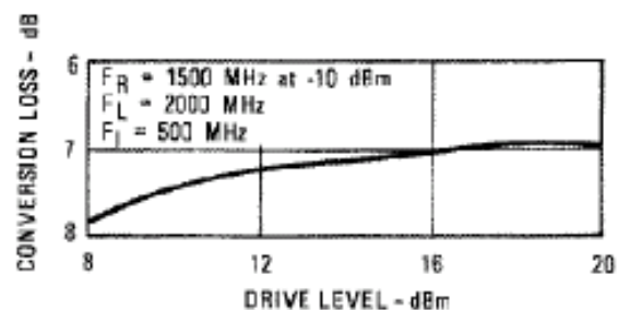
Conversion Loss
