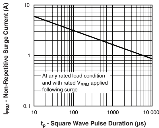
Fig. 5 - Maximum Non-Repulsive Surge Current
