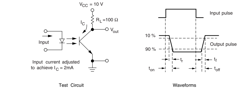
Fig. 1 - Switching Times
