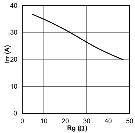
Fig. 14 - Typical Diode I_{RR} vs. R_G T_J = 125^\circ\text{C} ; I_F = 15\text{ A}
